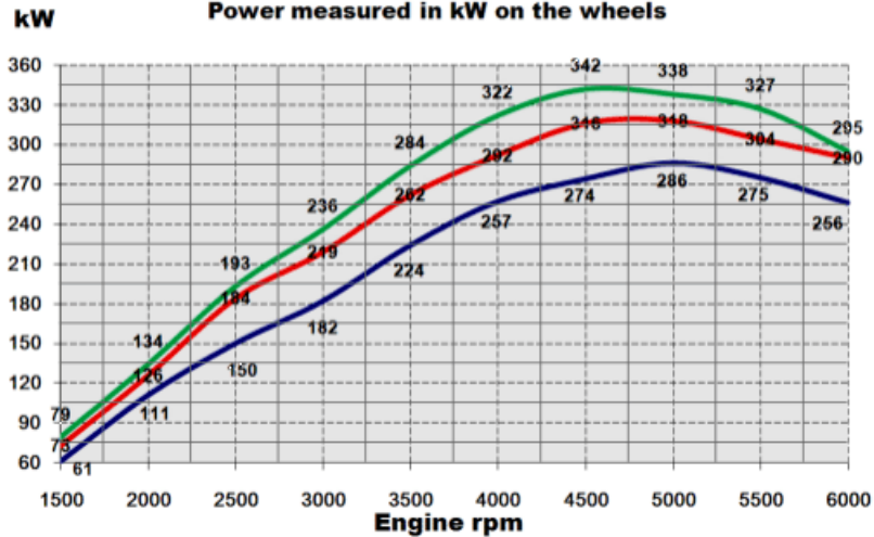
BMW E71 X6 xDrive 50i: De cat, Uni-Q Power measured in kW on the wheels
