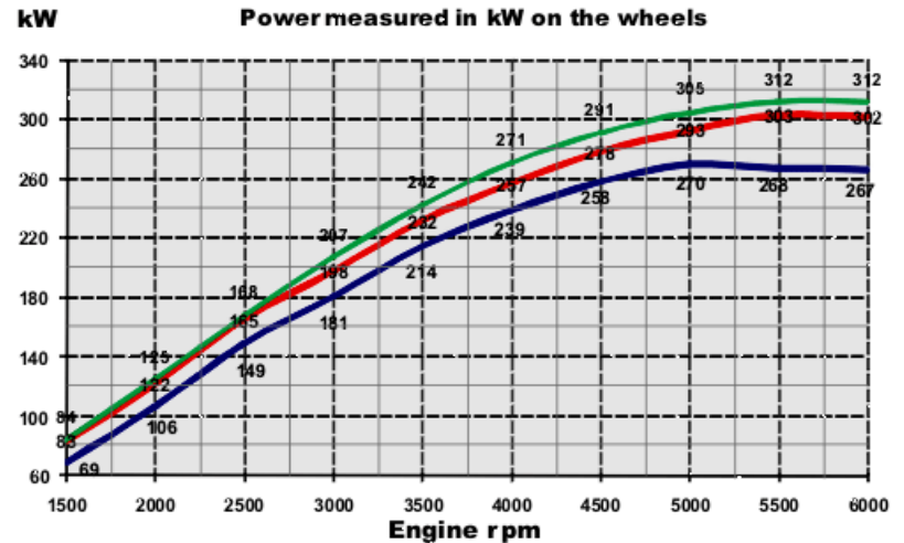
M/Benz E 55 AMG: Boost upgrade and Torco mapping Power measured in kW on the wheels
